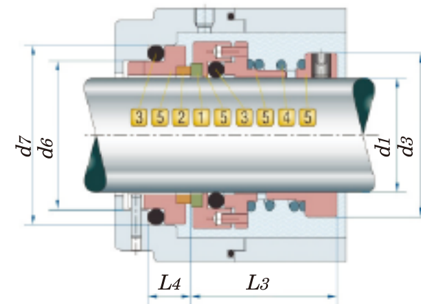
Type of counter ring
