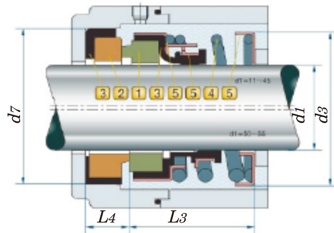
Single mechanical seal JX-108
