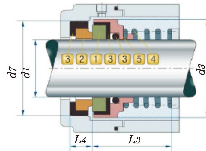
Single mechanical end seal with conical spring JX-101.
