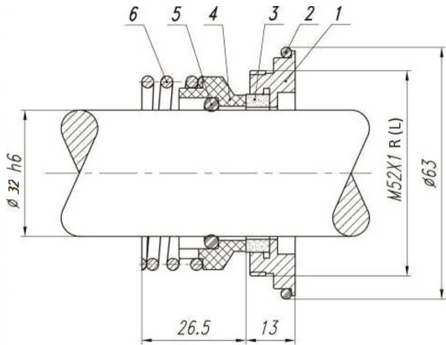
Single mechanical end seal JX-AL
