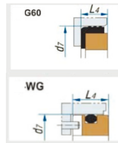
Mechanical seal JX-T1/FBC
