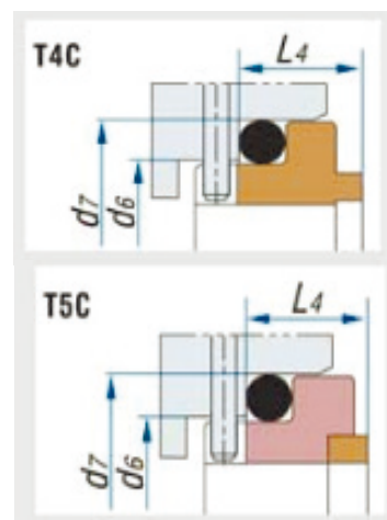
Type of counter ring
