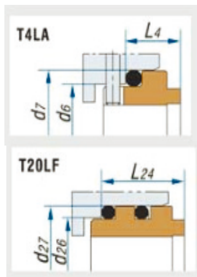
Type of counter ring
