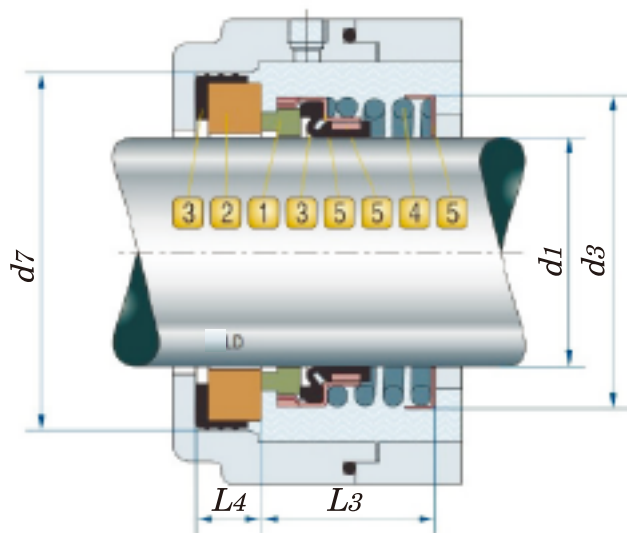
The mechanical end seal JX-560A
