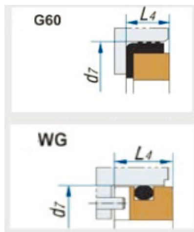
Mechanical seal JX-T2/FBD
