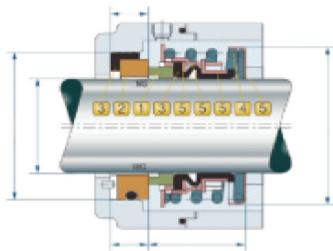
Type of counter ring
