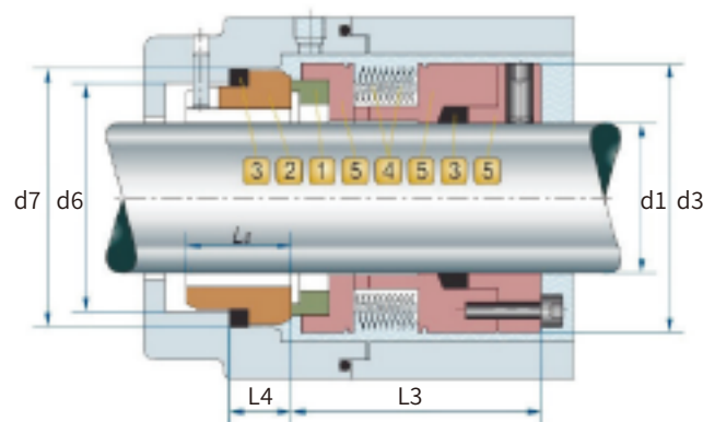
Type of counter ring
