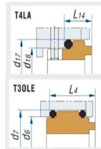
Type of counter ring
