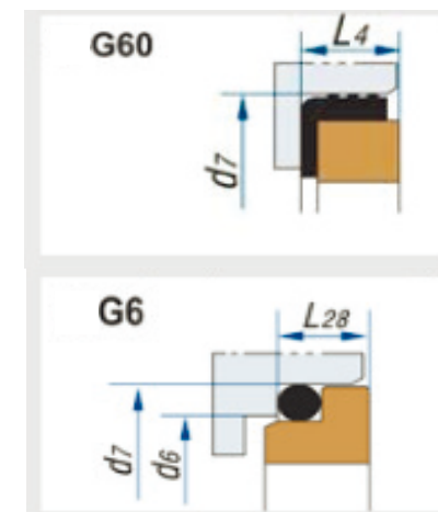
Mechanical seal JX-BIA
